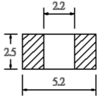
Recommend Land Pattern Dimensions
